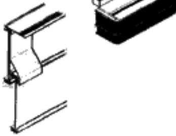
BACK VIEW OF UPPER VALANCE, DOUBLE VALANCE AND VALANCE HANGER
